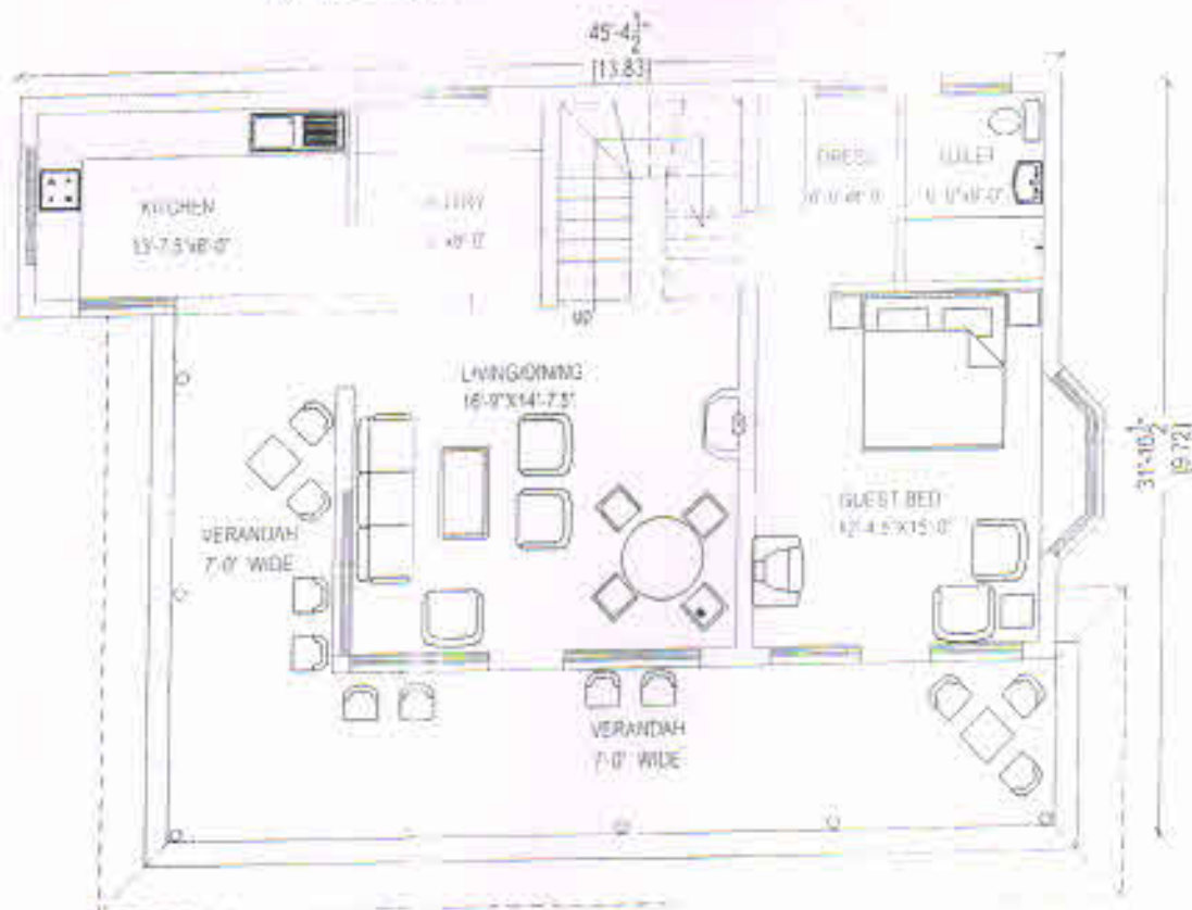
GROUND FLOOR PLAN COVD AREA = 1300 SQ FT
