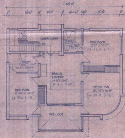
GROUND FLOOR (Lower level plan)
