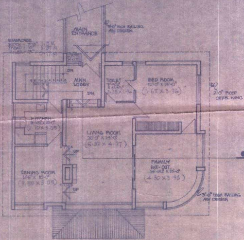
FIRST FLOOR (Entry level plan)
